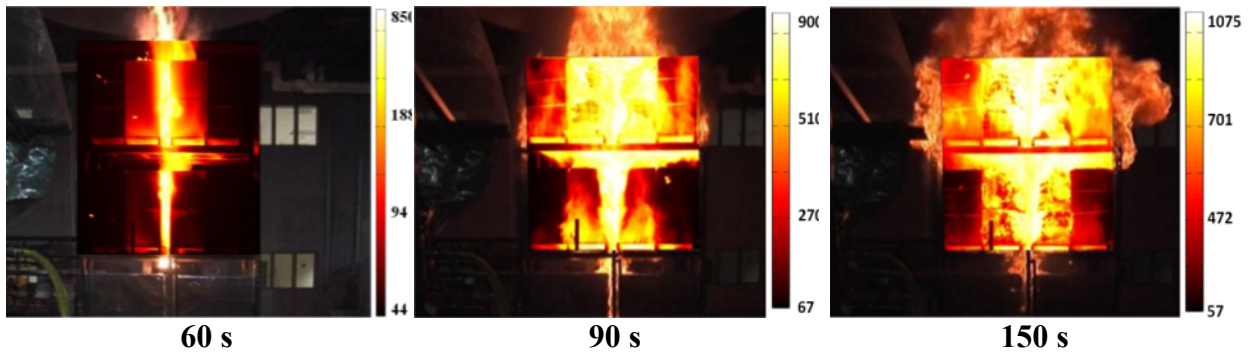
Figure 4-25: Registered images from CUP commodity - Test 9
