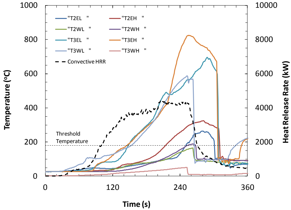
Figure A-14: Liner thermocouples - Test 7
