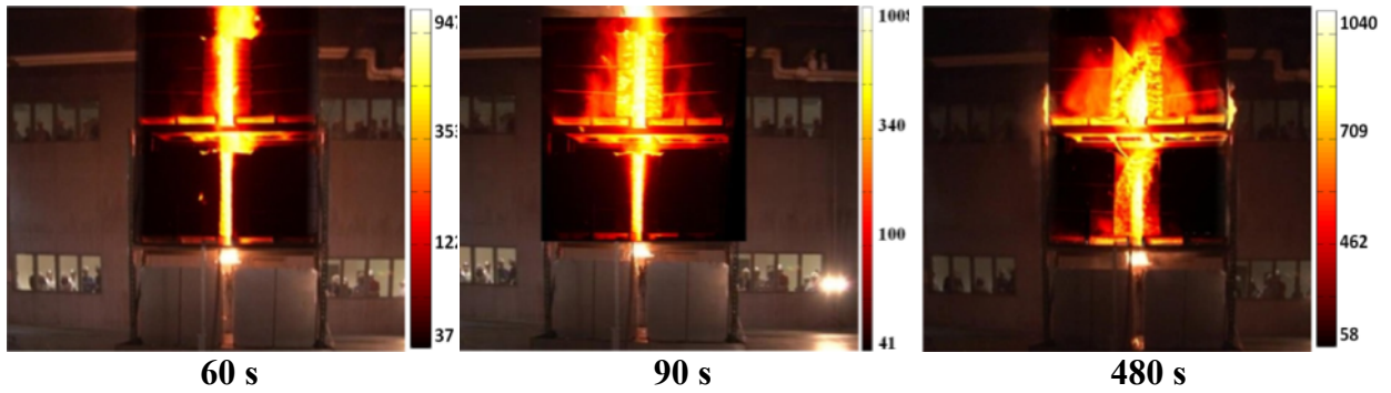
Figure 4-26: Registered images from Li-ion cylindrical cells - Test 11
