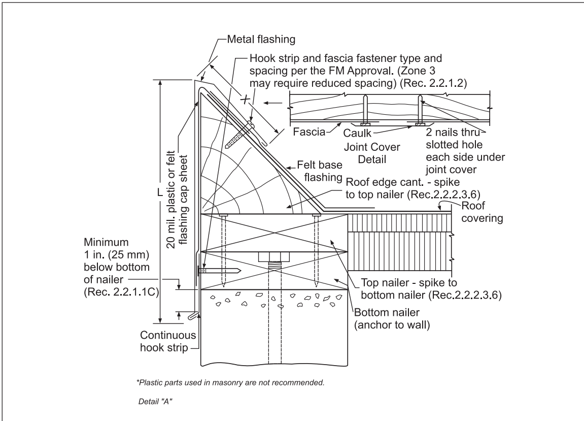
Fig. 3.1.1-4. Detail A from Figure 3.1.1-3
