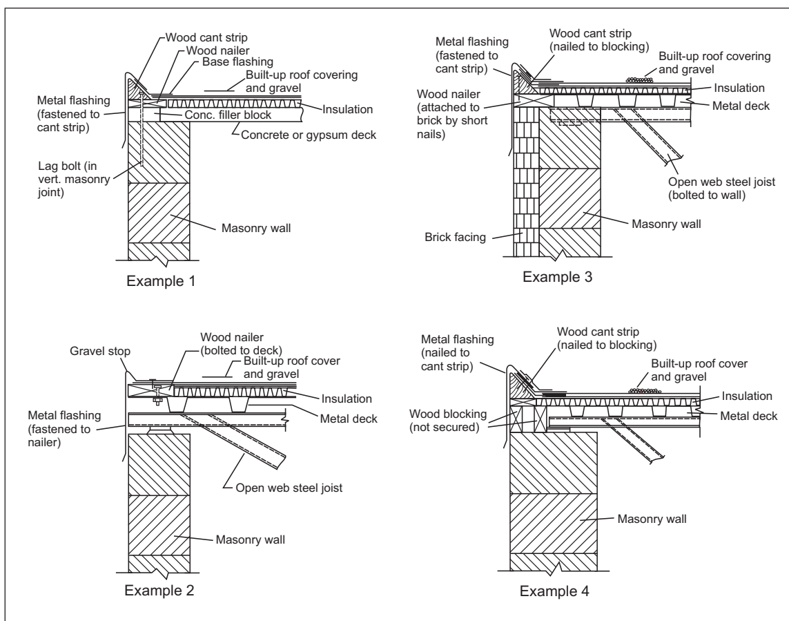
Fig. 3.6-1. Examples of perimeter flashing installations THAT ARE NOT RECOMMENDED
