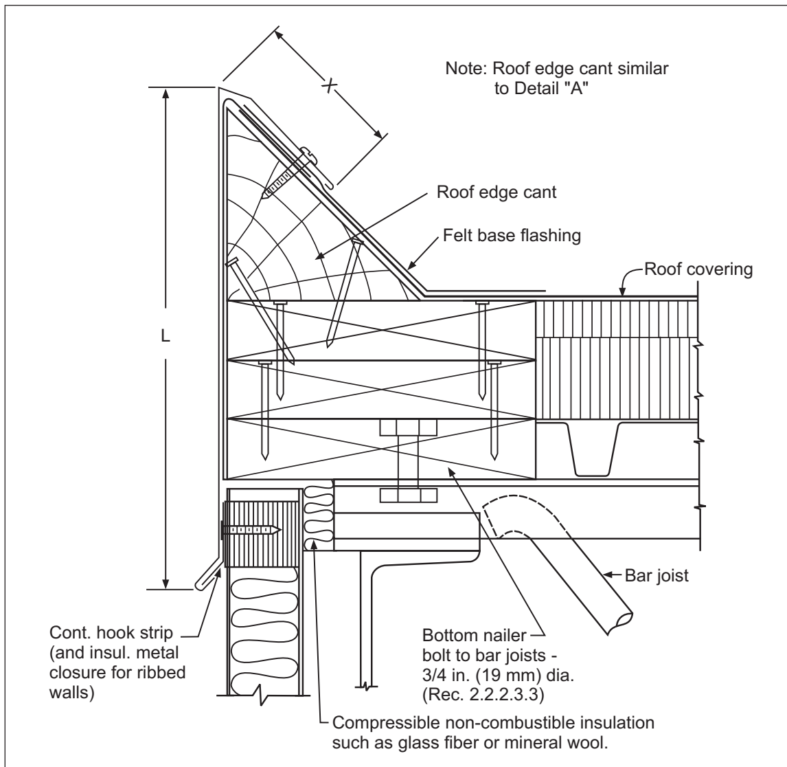
Fig. 3.1.3-1. Multi-ply roof with panel wall with roof edge cant, nailer bolted to roof joists
