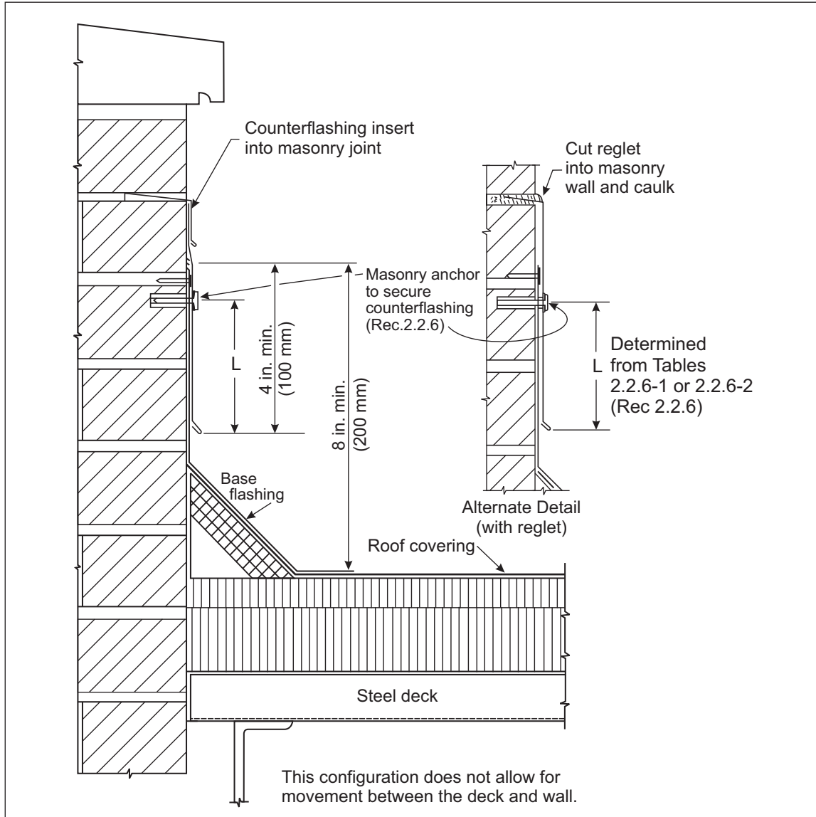
Fig. 3.1.2-1. Multi-ply roof cover with masonry wall with high parapet
