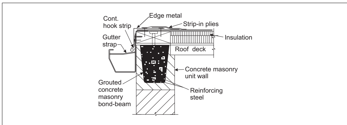
Fig. 3.1.6-1 Metal gutter with fascia flashing
