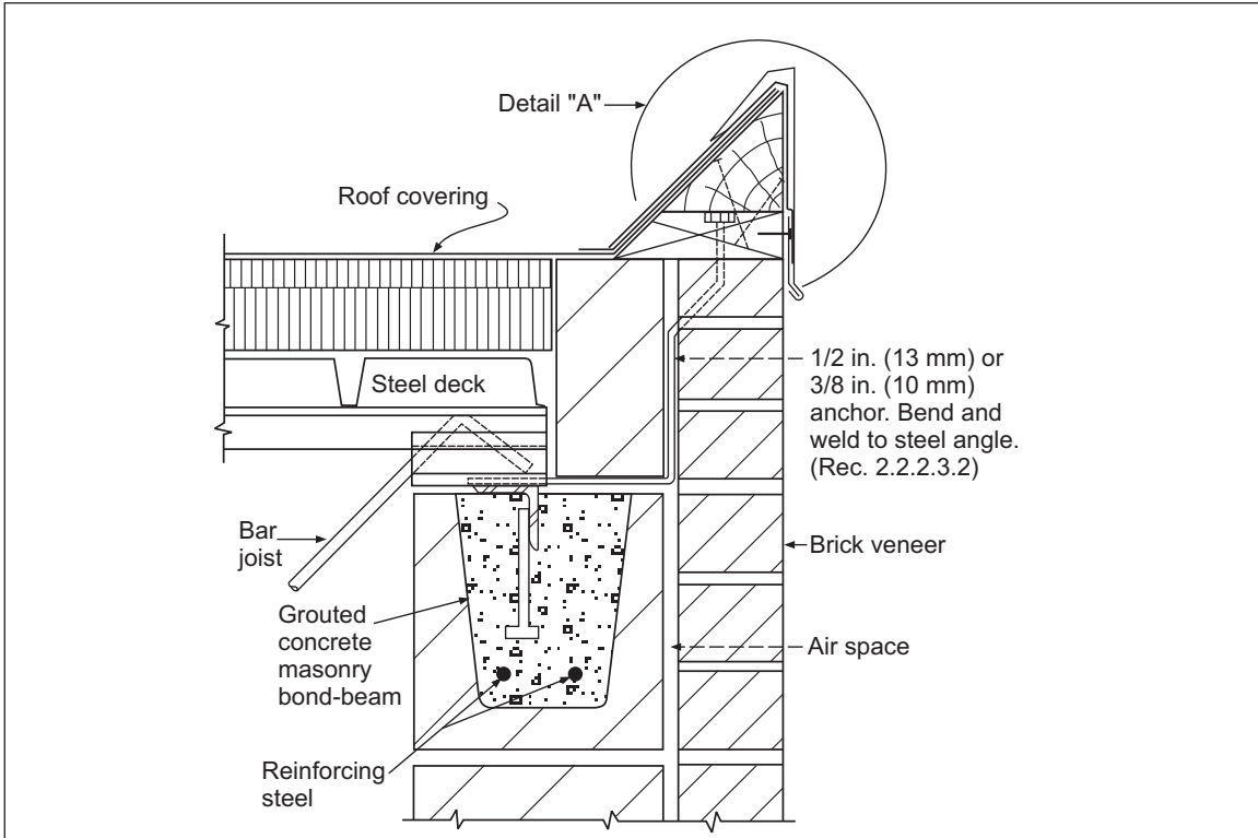
Fig. 3.1.1-3. Multi-ply roof cover with roof edge fascia cap (cant) flashing
